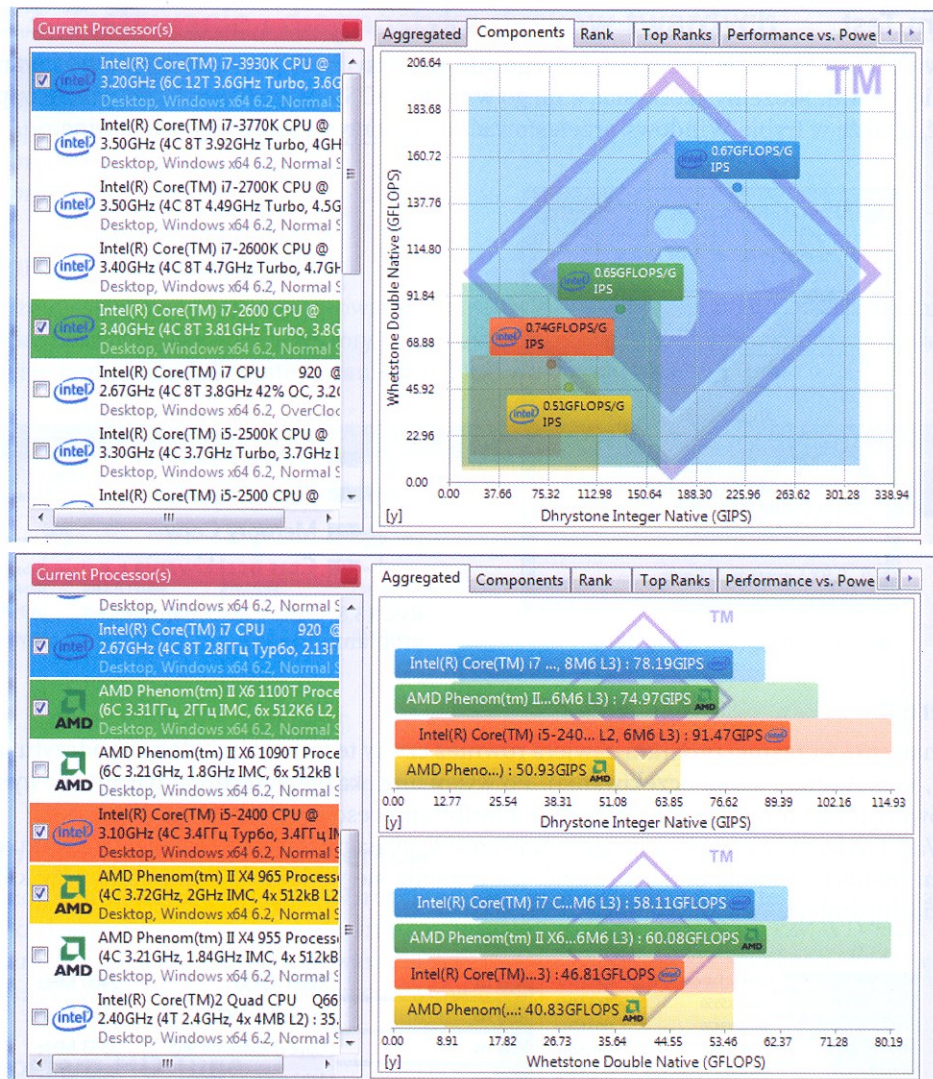
Rys. 13.6. Program Sandra Lite
